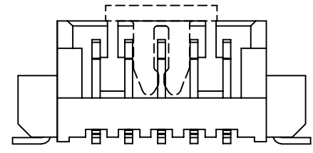
Odd Number
