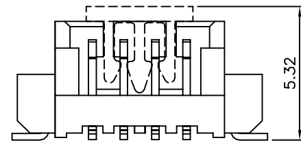
Dual Numbers
