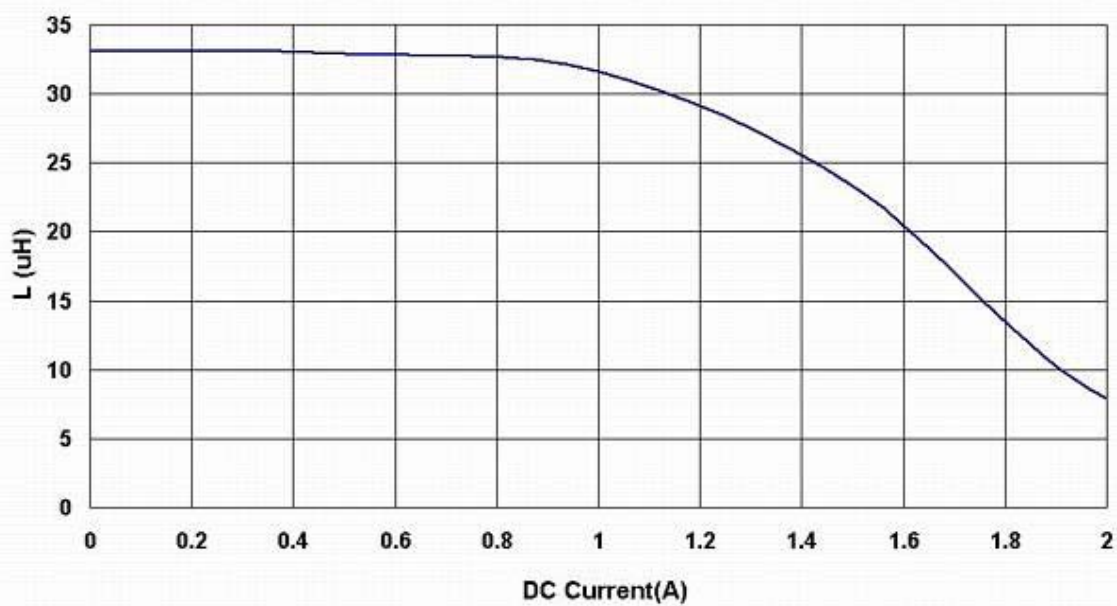
SCD0504T-330M-N1.1A
