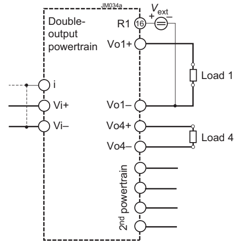
Fig. 19 Output adjust of V_{o1} and V_{o4} with an external voltage V_{ext} . The other outputs are not influenced.
