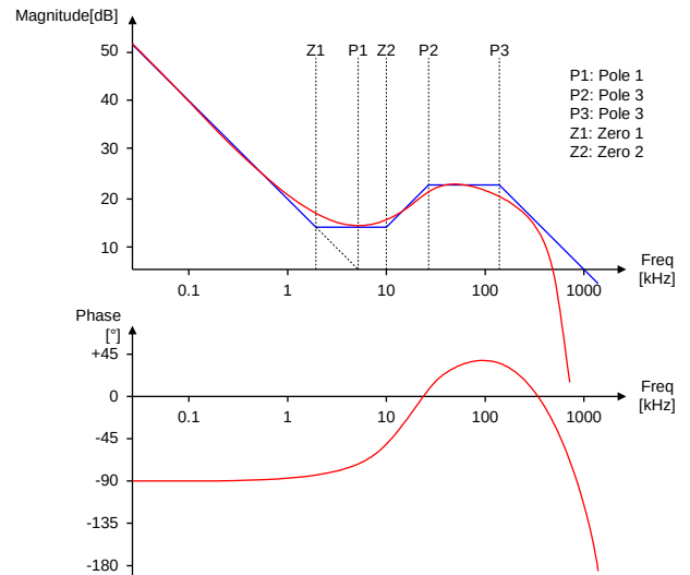
Figure 54. Transfer Function of PWM
