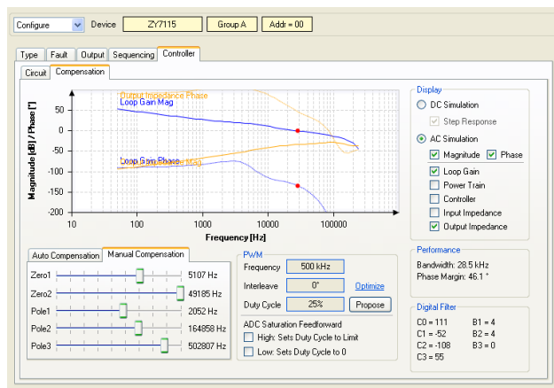
Figure 47. PWM Controller Window
