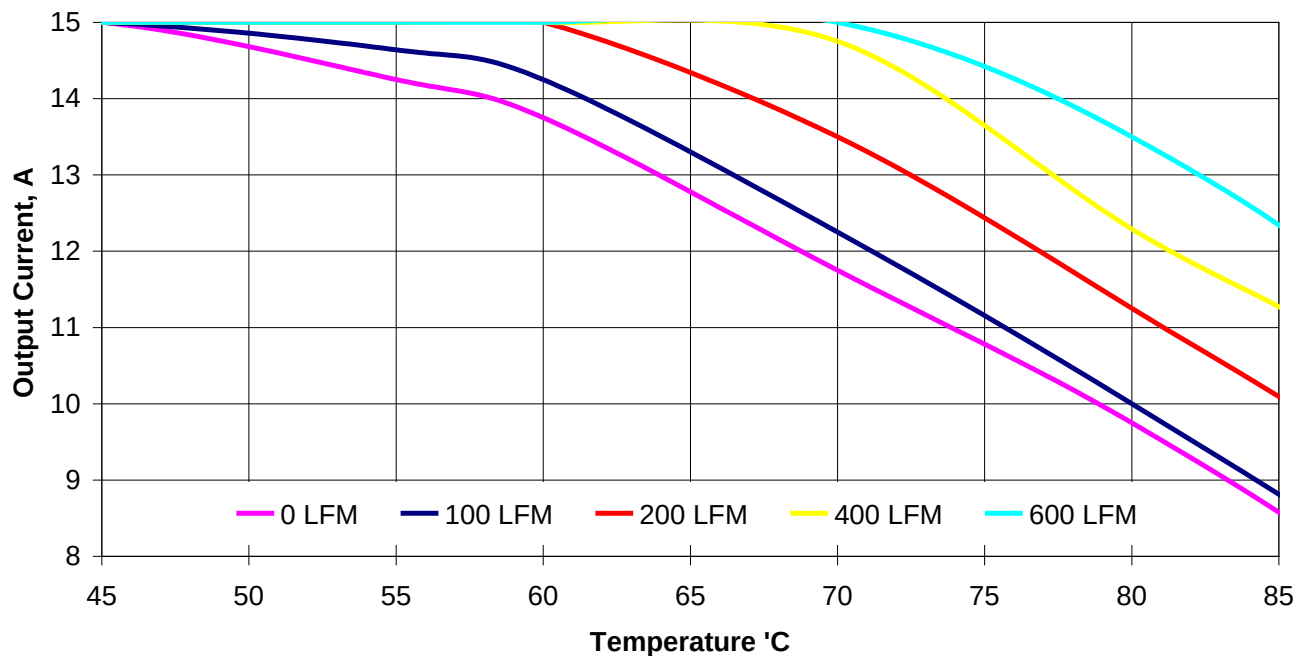
Figure 24. Thermal Derating Curves. Vin=13.2V, Vout=5.0V, Fsw=1MHz
