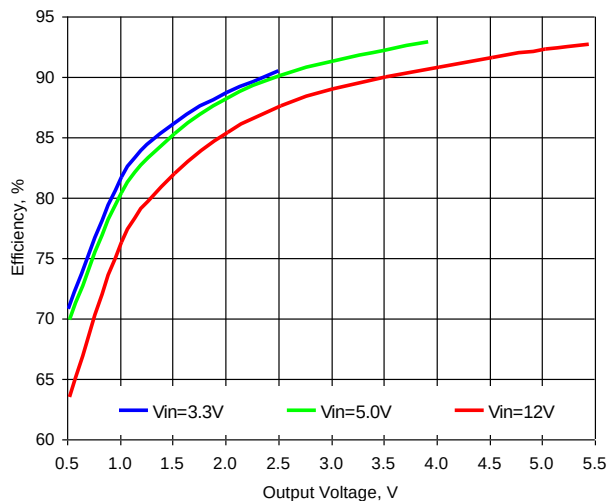
Figure 5. Efficiency vs. Output Voltage, Iout=15A, Fsw=500kHz
