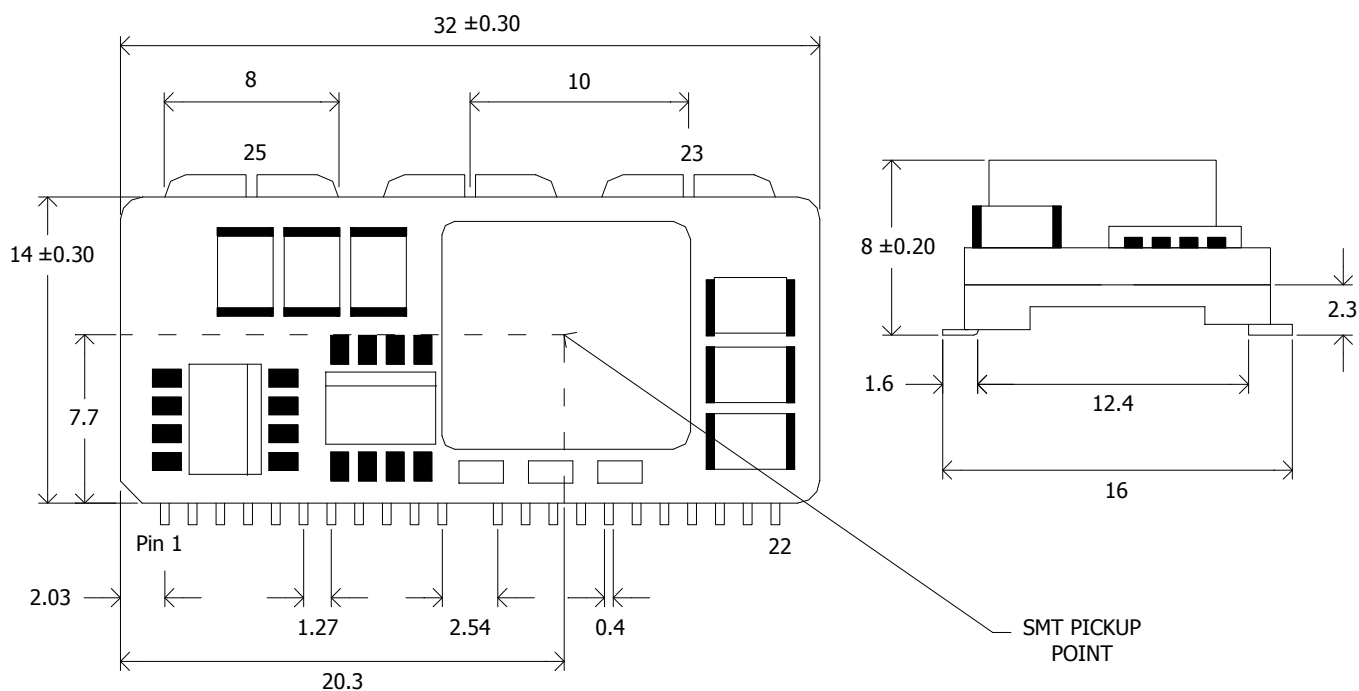
Figure 57. Mechanical Drawing
