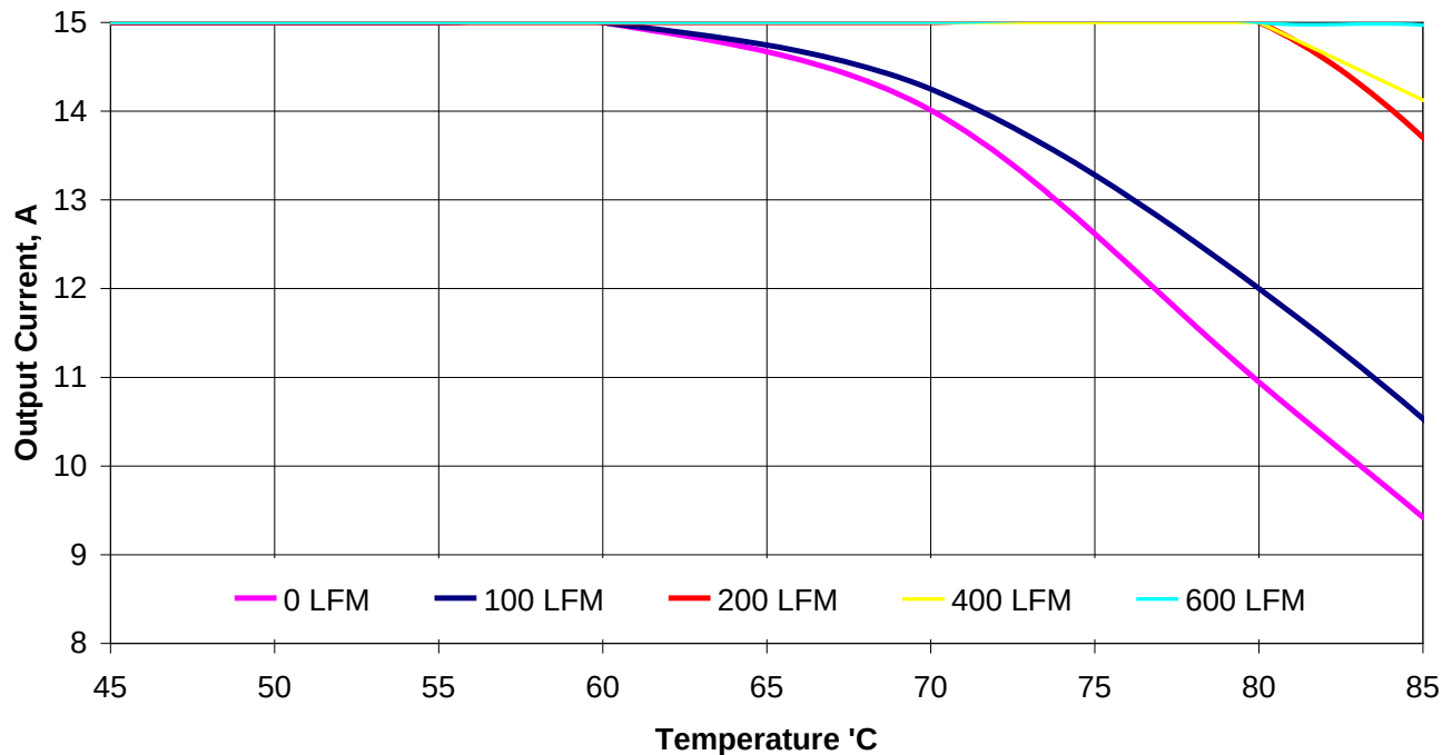
Figure 23. Thermal Derating Curves. Vin=13.2V, Vout=5.0V, Fsw=500kHz
