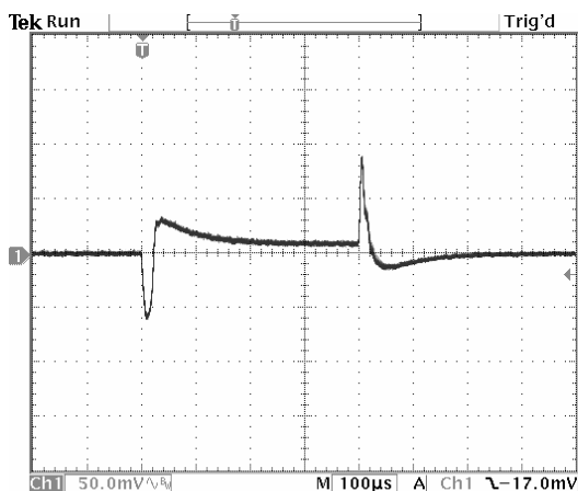
Figure 18. Vin=12V, Vout=1V. Bandwidth is 40kHz
