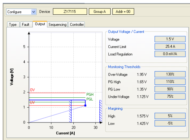
Figure 27. Output Configuration Window
