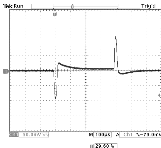
Figure 22. Vin=3V, Vout=1V. Bandwidth is 30kHz
