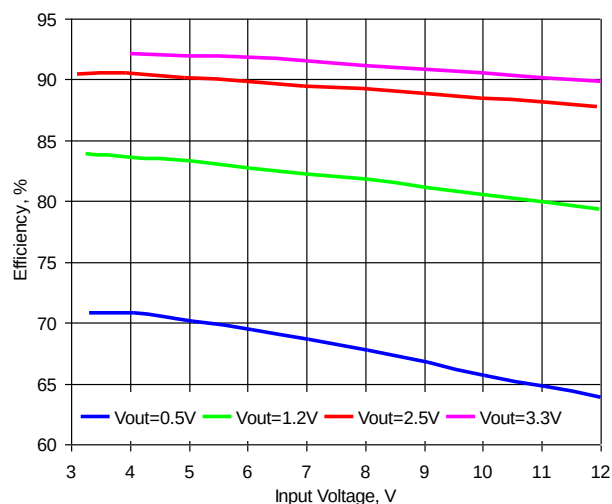
Figure 6. Efficiency vs. Input Voltage. Iout=15A, Fsw=500kHz
