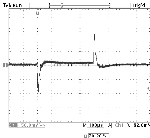
Figure 21. Vin=5V, Vout=2.5V. Bandwidth is 40kHz
