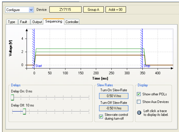
Figure 32. Sequencing/Tracking Window
