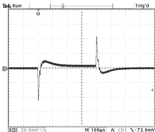
Figure 19. Vin=12V, Vout=5V. Bandwidth is 40kHz
