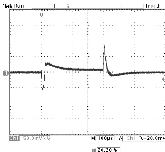
Figure 20. Vin=5V, Vout=1V. Bandwidth is 40kHz
