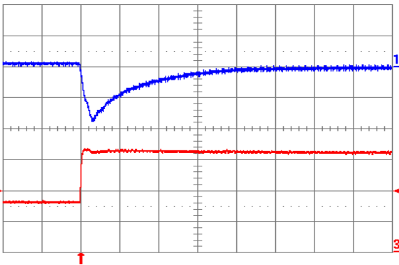
Fig. 1.5V.7: Output voltage response for V_{out} = 1.5 V to positive load current step change from 8 A to 16 A with slew rate of 5 \text{ A}/\mu\text{s} at V_{in} = 5 V. Top trace: output voltage (100 mV/div.); Bottom trace: load current (5 A/div.). C_o = 100 \mu\text{F} ceramic. Time scale: 20 \mu\text{s}/\text{div} .
