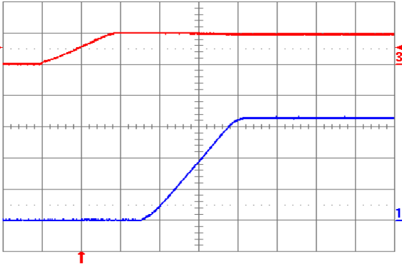
Fig. 3.3V.5: Turn-on transient for V_{out} = 3.3 V with application of V_{in} at full rated load current (resistive) and 100 \mu\text{F} external capacitance at V_{in} = 5 V. Top trace: V_{in} (5 V/div.); Bottom trace: output voltage (1 V/div.); Time scale: 2 ms/div.
