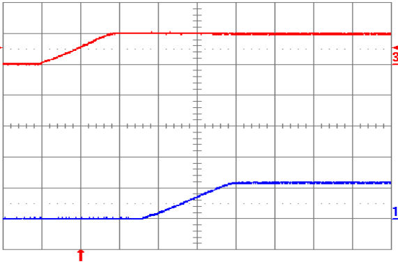
Fig. 1.2V.5: Turn-on transient for V_{out} = 1.2 V with application of V_{in} at full rated load current (resistive) and 100 \mu\text{F} external capacitance at V_{in} = 5 V. Top trace: V_{in} (5 V/div.); Bottom trace: output voltage (1 V/div.); Time scale: 2 ms/div.
