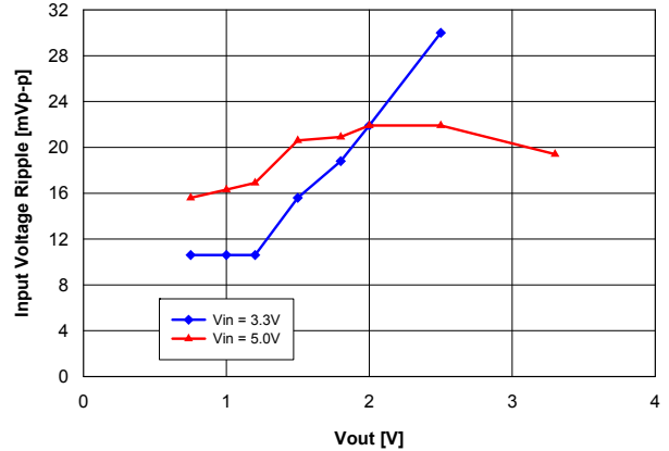
Fig. B: Input Voltage Ripple, C_{IN} = 470 \mu\text{F} polymer + 2 x 47 \mu\text{F} ceramic.
