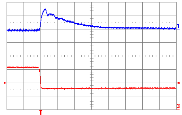
Fig. 3.3V.8: Output voltage response for V_{out} = 3.3 V to negative load current step change from 16 A to 8 A with slew rate of -5 \text{ A}/\mu\text{s} at V_{in} = 5 V. Top trace: output voltage (100 mV/div.); Bottom trace: load current (5 A/div.). C_o = 100 \mu\text{F} ceramic. Time scale: 20 \mu\text{s}/\text{div} .
