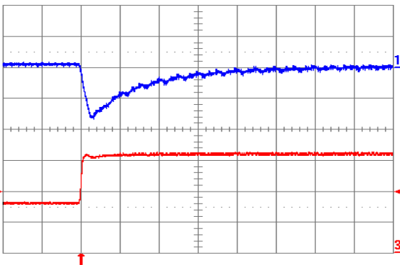
Fig. 1.2V.6: Output voltage response for V_{out} = 1.2 V to positive load current step change from 8 A to 16 A with slew rate of 5 \text{ A}/\mu\text{s} at V_{in} = 5 V. Top trace: output voltage (100 mV/div.); Bottom trace: load current (5 A/div.). C_o = 100 \mu\text{F} ceramic. Time scale: 20 \mu\text{s}/\text{div} .
