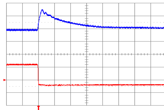
Fig. 2.0V.8: Output voltage response for V_{out} = 2.0 V to negative load current step change from 16 A to 8 A with slew rate of -5\text{ A}/\mu\text{s} at V_{in} = 5 V. Top trace: output voltage (100 mV/div.); Bottom trace: load current (5 A/div.). C_o = 100\mu\text{F} ceramic. Time scale: 20 \mu\text{s} /div.
