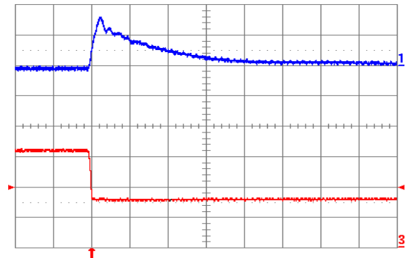
Fig. 2.5V.8: Output voltage response for V_{out} = 2.5 V to negative load current step change from 16 A to 8 A with slew rate of -5 \text{ A}/\mu\text{s} at V_{in} = 5 V. Top trace: output voltage (100 mV/div.); Bottom trace: load current (5 A/div.). C_o = 100 \mu\text{F} ceramic. Time scale: 20 \mu\text{s} /div.
