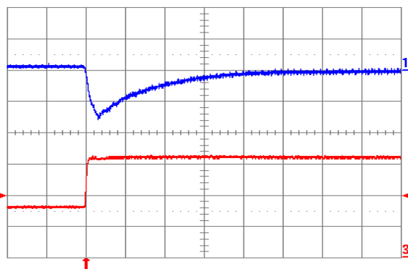
Fig. 2.0V.7: Output voltage response for V_{out} = 2.0 V to positive load current step change from 8 A to 16 A with slew rate of 5\text{ A}/\mu\text{s} at V_{in} = 5 V. Top trace: output voltage (100 mV/div.); Bottom trace: load current (5 A/div.). C_o = 100\mu\text{F} ceramic. Time scale: 20 \mu\text{s} /div.
