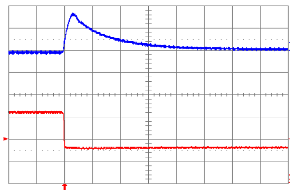
Fig. 1.0V.8: Output voltage response for V_{out} = 1.0 V to negative load current step change from 16 A to 8 A with slew rate of -5 \text{ A}/\mu\text{s} at V_{in} = 5 V. Top trace: output voltage (100 mV/div.); Bottom trace: load current (5 A/div.). C_o = 100 \mu\text{F} ceramic + 1 \mu\text{F} ceramic. Time scale: 20 \mu\text{s}/\text{div} .
