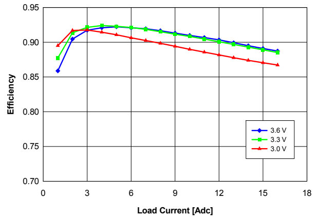
Fig. 2.0V.4: Efficiency vs. load current and input voltage for V_{out} = 2.0 V converter mounted horizontally with air flowing at a rate of 200 LFM (1 m/s) and T_a = 25 °C.
