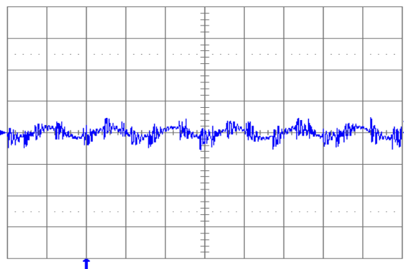
Fig. 2.0V.6: Output voltage ripple (20 mV/div.) at full rated load current into a resistive load with external capacitance 100\mu\text{F} ceramic + 1\mu\text{F} ceramic and V_{in} = 5 V for V_{out} = 2.0 V. Time scale: 2 \mu\text{s} /div.
