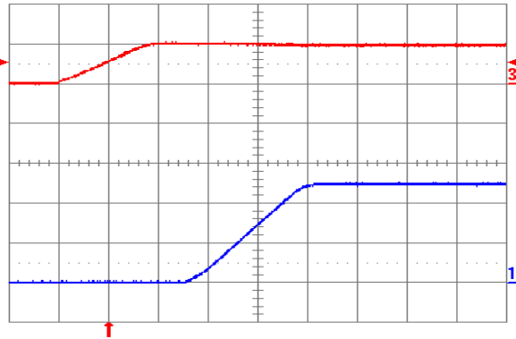
Fig. 2.5V.5: Turn-on transient for V_{out} = 2.5 V with application of V_{in} at full rated load current (resistive) and 100 \mu\text{F} external capacitance at V_{in} = 5 V. Top trace: V_{in} (5 V/div.); Bottom trace: output voltage (1 V/div.); Time scale: 2 ms/div.
