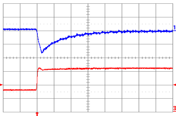
Fig. 1.0V.7: Output voltage response V_{out} = 1.0 V to positive load current step change from 8 A to 16 A with slew rate of 5 \text{ A}/\mu\text{s} at V_{in} = 5 V. Top trace: output voltage (100 mV/div.); Bottom trace: load current (5 A/div.). C_o = 100 \mu\text{F} ceramic + 1 \mu\text{F} ceramic. Time scale: 20 \mu\text{s}/\text{div} .
