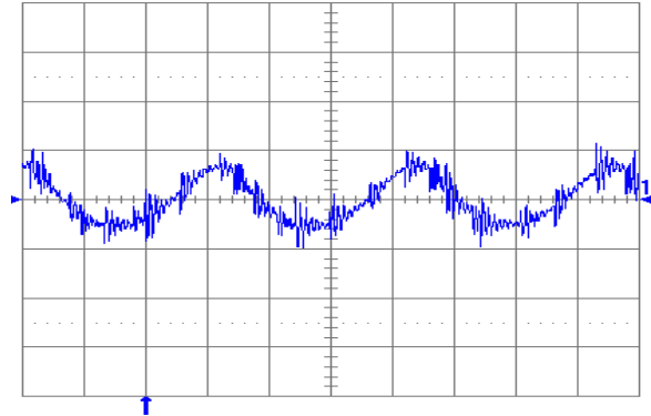
Fig. 3.3V.6: Output voltage ripple (20 mV/div.) at full rated load current into a resistive load with external capacitance 100 \mu\text{F} ceramic + 1 \mu\text{F} ceramic and V_{in} = 5 V for V_{out} = 3.3 V. Time scale: 2 \mu\text{s}/\text{div} .
