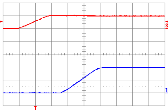
Fig. 2.0V.5: Turn-on transient for V_{out} = 2.0 V with application of V_{in} at full rated load current (resistive) and 100\mu\text{F} external capacitance at V_{in} = 5 V. Top trace: V_{in} (5 V/div.); Bottom trace: output voltage (1 V/div.); Time scale: 2 ms/div.
