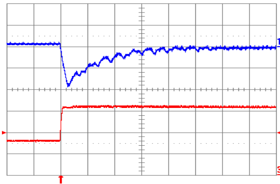
Fig. 3.3V.7: Output voltage for V_{out} = 3.3 V to positive load current step change from 8 A to 16 A with slew rate of 5 \text{ A}/\mu\text{s} at V_{in} = 5 V. Top trace: output voltage (100 mV/div.); Bottom trace: load current (5 A/div.). C_o = 100 \mu\text{F} ceramic. Time scale: 20 \mu\text{s}/\text{div} .
