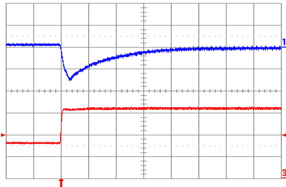
Fig. 1.8V.7: Output voltage response for V_{out} = 1.8 V to positive load current step change from 8 A to 16 A with slew rate of 5\text{ A}/\mu\text{s} at V_{in} = 5 V. Top trace: output voltage (100 mV/div.); Bottom trace: load current (5 A/div.). C_o = 100\mu\text{F} ceramic. Time scale: 20 \mu\text{s} /div.
