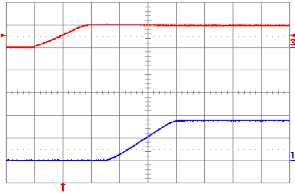
Fig. 1.8V.5: Turn-on transient for V_{out} = 1.8 V with application of V_{in} at full rated load current (resistive) and 100\mu\text{F} external capacitance at V_{in} = 5 V. Top trace: V_{in} (5 V/div.); Bottom trace: output voltage (1V/div.); Time scale: 2 ms/div.
