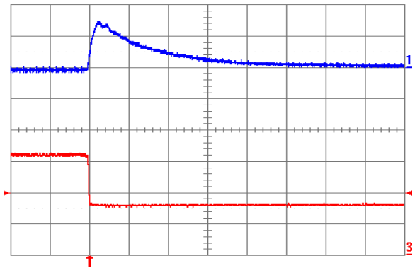
Fig. 1.5V.8: Output voltage response for V_{out} = 1.5 V to negative load current step change from 16 A to 8 A with slew rate of -5 \text{ A}/\mu\text{s} at V_{in} = 5 V. Top trace: output voltage (100 mV/div.); Bottom trace: load current (5 A/div.). C_o = 100 \mu\text{F} ceramic. Time scale: 20 \mu\text{s}/\text{div} .
