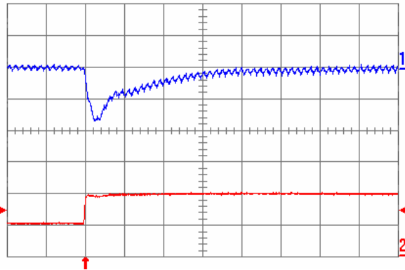
Fig. 1.5V.7: Output voltage response for V_{out} = 1.5\text{ V} to positive load current step change from 5\text{ A} to 10\text{ A} with slew rate of 5\text{ A}/\mu\text{s} at V_{in} = 5\text{ V} . Top trace: output voltage ( 100\text{ mV/div.} ); Bottom trace: load current ( 5\text{ A/div.} ). C_o = 100\text{ }\mu\text{F} ceramic + 1\text{ }\mu\text{F} ceramic. Time scale: 20\text{ }\mu\text{s/div.}
