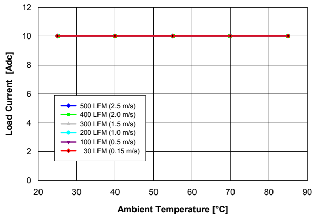
Fig. 2.5V.2: Available load current vs. ambient temperature and airflow rates for V_{out} = 2.5 V converter mounted horizontally with V_{in} = 5 V, and maximum MOSFET temperature \leq 120 °C.
