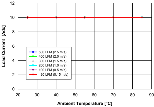
Fig. 1.8V.1: Available load current vs. ambient temperature and airflow rates for Vout = 1.8 V converter mounted vertically with Vin = 5 V, and maximum MOSFET temperature ≤ 120 °C.
