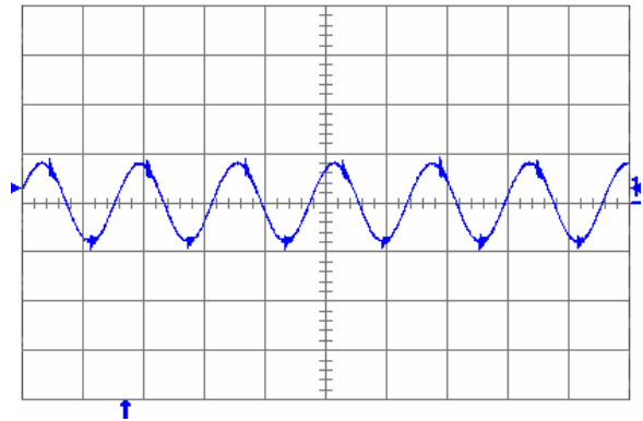
Fig. 1.8V.6: Output voltage ripple (20 mV/div.) at full rated load current into a resistive load with external capacitance 100 \mu\text{F} ceramic + 1 \mu\text{F} ceramic and V_{in} = 5 V for V_{out} = 1.8 V. Time scale: 2 \mu\text{s}/\text{div} .
