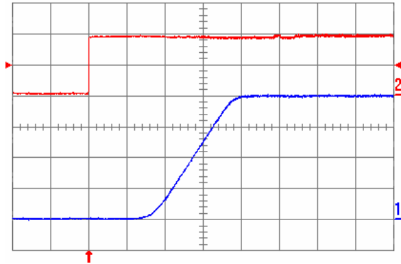
Fig. 2.0V.5: Turn-on transient for V_{out} = 2.0 V with the application of Enable signal at full rated load current (resistive) and 100 \mu\text{F} external capacitance at V_{in} = 5 V. Top trace: Enable signal (2 V/div.); Bottom trace: output voltage (500 mV/div.); Time scale: 2 ms/div.
