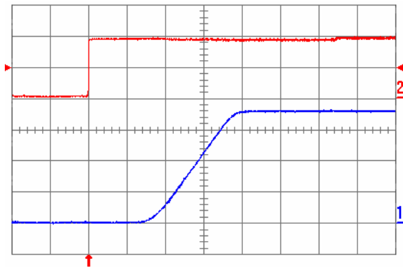
Fig. 1.8V.5: Turn-on transient for V_{out} = 1.8 V with the application of Enable signal at full rated load current (resistive) and 100 \mu\text{F} external capacitance at V_{in} = 5 V. Top trace: Enable signal (2 V/div.); Bottom trace: output voltage (500 mV/div.); Time scale: 2 ms/div.
