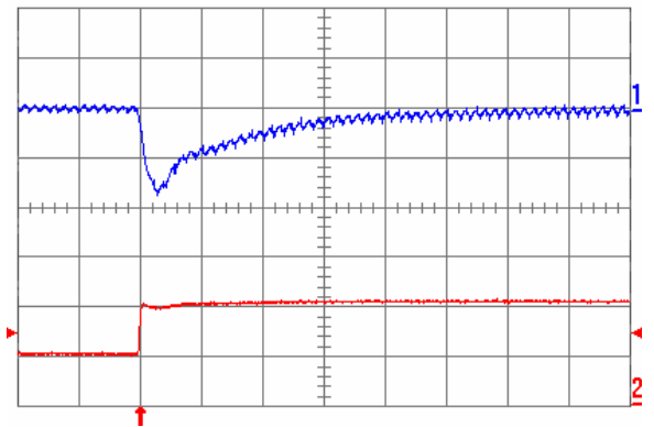
Fig. 1.2V.6: Output voltage response for V_{out} = 1.2 V to positive load current step change from 5 A to 10 A with slew rate of 5 A/ \mu s at V_{in} = 5 V. Top trace: output voltage (100 mV/div.); Bottom trace: load current (5 A/div.). C_o = 100 \mu F ceramic + 1 \mu F ceramic. Time scale: 20 \mu s/div.
