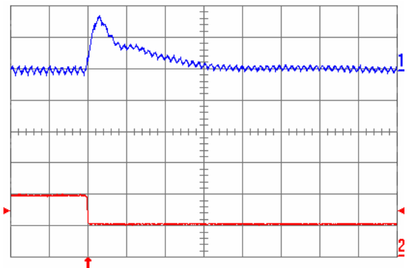
Fig. 1.8V.8: Output voltage response for V_{out} = 1.8 V to negative load current step change from 10 A to 5 A with slew rate of -5 \text{ A}/\mu\text{s} at V_{in} = 5 V. Top trace: output voltage (100 mV/div.); Bottom trace: load current (5 A/div.). C_o = 100 \mu\text{F} ceramic + 1 \mu\text{F} ceramic. Time scale: 20 \mu\text{s}/\text{div} .
