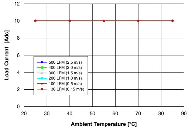
Fig. 1.8V.2: Available load current vs. ambient temperature and airflow rates for Vout = 1.8 V converter mounted horizontally with Vin = 5 V, and maximum MOSFET temperature ≤ 120 °C.
