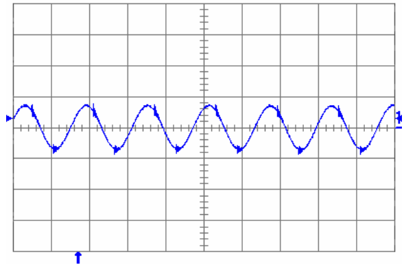
Fig. 1.5V.6: Output voltage ripple ( 20\text{ mV/div.} ) at full rated load current into a resistive load with external capacitance 100\text{ }\mu\text{F} ceramic + 1\text{ }\mu\text{F} ceramic and V_{in} = 5\text{ V} for V_{out} = 1.5\text{ V} . Time scale: 2\text{ }\mu\text{s/div.}
