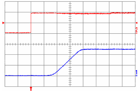
Fig. 2.5V.5: Turn-on transient for V_{out} = 2.5 V with the application of Enable signal at full rated load current (resistive) and 100 \mu\text{F} external capacitance at V_{in} = 5 V. Top trace: Enable signal (2 V/div.); Bottom trace: output voltage (1 V/div.); Time scale: 2 ms/div.
