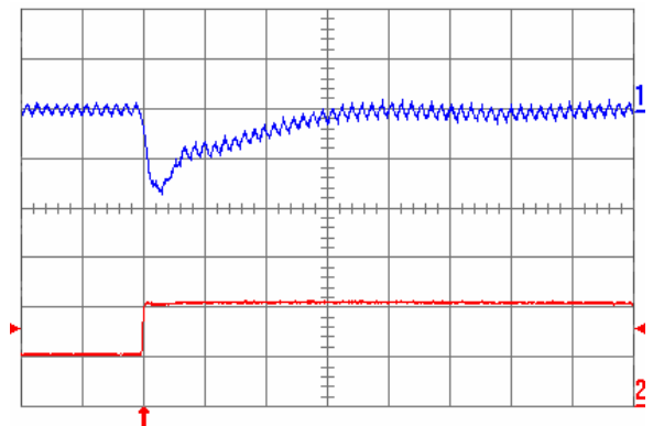
Fig. 2.5V.7: Output voltage response for V_{out} = 2.5 V to positive load current step change from 5 A to 10 A with slew rate of 5 \text{ A}/\mu\text{s} at V_{in} = 5 V. Top trace: output voltage (100 mV/div.); Bottom trace: load current (5 A/div.). C_o = 100 \mu\text{F} ceramic + 1 \mu\text{F} ceramic. Time scale: 20 \mu\text{s}/\text{div} .
