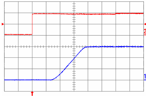
Fig. 1.5V.5: Turn-on transient for V_{out} = 1.5\text{ V} with the application of Enable signal at full rated load current (resistive) and 100\text{ }\mu\text{F} external capacitance at V_{in} = 5\text{ V} . Top trace: Enable signal ( 2\text{ V/div.} ); Bottom trace: output voltage ( 500\text{ mV/div.} ); Time scale: 2\text{ ms/div.}
