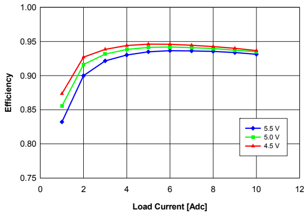
Fig. 2.5V.3: Efficiency vs. load current and input voltage for V_{out} = 2.5\text{ V} converter mounted vertically with air flowing at a
