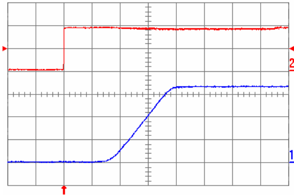
Fig. 3.3V.5: Turn-on transient for V_{out} = 3.3 V with the application of Enable signal at full rated load current (resistive) and 100 \mu\text{F} external capacitance at V_{in} = 5 V. Top trace: Enable signal (2 V/div.); Bottom trace: output voltage (1 V/div.); Time scale: 2 ms/div.
