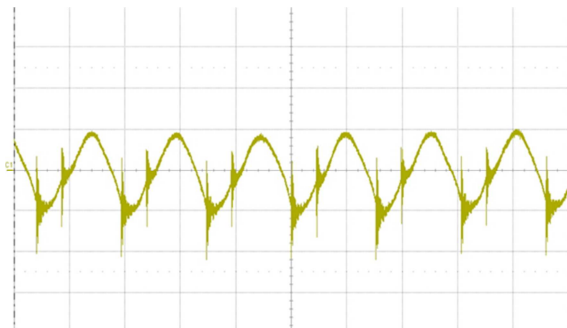
Fig. 13: Output voltage ripple (20 mV/div.) at full rated load current into a resistive load with C_o = 10 \mu\text{F} tantalum + 1 \mu\text{F} ceramic and V_{in} = 48 \text{ V} . Time scale: 2 \mu\text{s}/\text{div}
