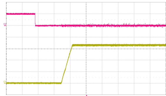
Fig. 12: Output voltage response to load current step-change (10A – 15A – 10A) at V_{in} = 48 \text{ V} . Current slew rate: 0.1 \text{ A}/\mu\text{s} . C_o = 4700\mu\text{F} E-cap + 1 \mu\text{F} ceramic + 10 \mu\text{F} tantalum. Time scale: 500 \mu\text{s}/\text{div} .
