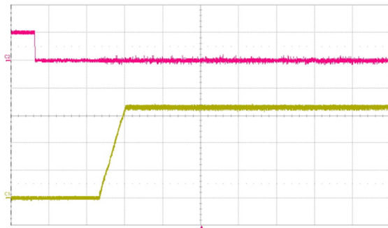
Fig. 11: Output voltage response to load current step-change (10 A – 15 A – 10 A) at V_{in} = 48 \text{ V} . Current slew rate: 0.1 \text{ A}/\mu\text{s} . C_o = 470\mu\text{F} E-cap + 1 \mu\text{F} ceramic + 10 \mu\text{F} tantalum. Time scale: 500 \mu\text{s}/\text{div} .
