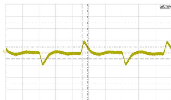
Fig. 11: Output voltage response to load current step-change (7A – 10.5 A – 7 A) at V_{in} = 48\text{ V} . Current slew rate: 0.1 A/ \mu\text{s} . C_o = 470\mu\text{F} E-cap + 1 \mu\text{F} ceramic + 10 \mu\text{F} tantalum. Time scale: 100 \mu\text{s} /div.
