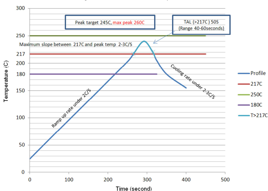
Fig. 21: Lead Free solder reflow profile:
