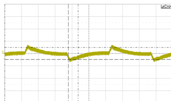
Fig. 12: Output voltage response to load current step-change (7A – 10.5A – 7A) at V_{in} = 48\text{ V} . Current slew rate: 0.1 A/ \mu\text{s} . C_o = 4700\mu\text{F} E-cap + 1 \mu\text{F} ceramic + 10 \mu\text{F} tantalum. Time scale: 500 \mu\text{s} /div.
