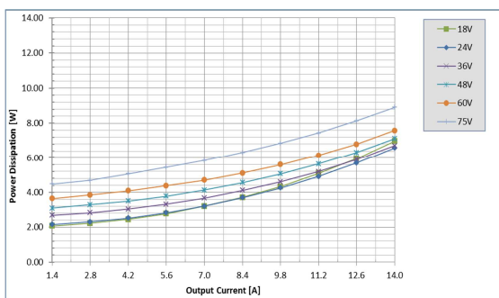
Fig. 8: Power dissipation vs. load current and input voltage for UIS48T14050 converter w/o baseplate mounted vertically with air flowing from pin 3 to pin 1 at a rate of 300 LFM (1.5 m/s) and T_a = 25^\circ\text{C} .
