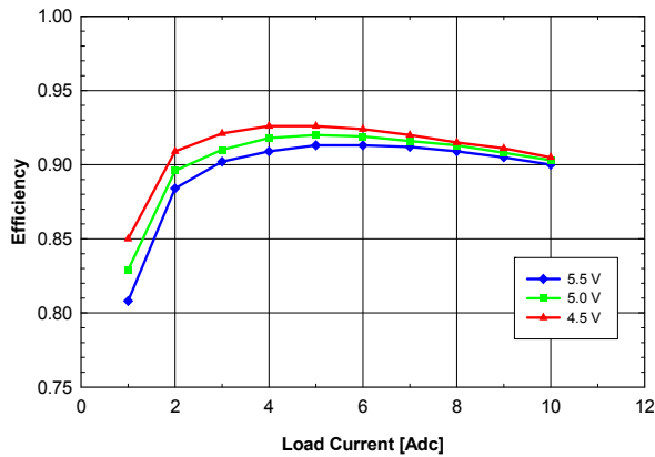
Fig. 1.5V.3: Efficiency vs. load current and input voltage for V out = 1.5V converter mounted vertically with air flowing from pin 10 to pin 1 at a rate of 200 LFM (1m/s) and T a = 25°C.
