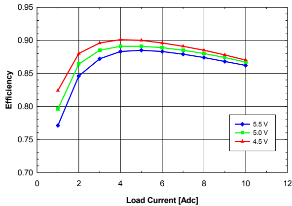
Fig. 1.0V.3: Efficiency vs. load current and input voltage for V out = 1.0V converter mounted vertically with air flowing from pin 10 to pin 1 at a rate of 200 LFM (1m/s) and T a = 25°C.
