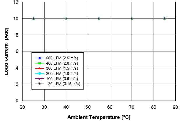
Fig. 1.0V.2: Available load current vs. ambient temperature and airflow rates for V out = 1.0V converter mounted horizontally with air flowing from pin 10 to pin 1, and maximum MOSFET temperature ≤ 120°C.
