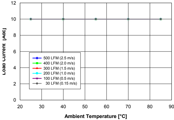
Fig. 1.0V.1: Available load current vs. ambient temperature and airflow rates for V out = 1.0V converter mounted vertically with air flowing from pin 10 to pin 1, and maximum MOSFET temperature ≤ 120°C.
