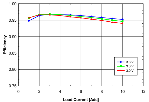
Fig. 2.5V.4: Efficiency vs. load current and input voltage for V_{out} = 2.5V converter mounted vertically with air flowing from pin 10 to pin 1 at a rate of 200 LFM (1m/s) and T_a = 25^{\circ}C .
