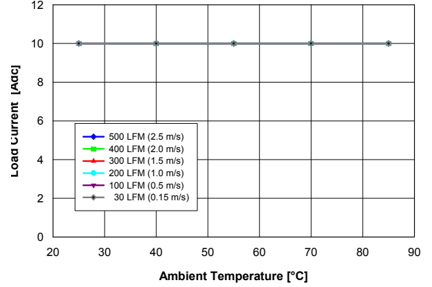
Fig. 1.2V.2: Available load current vs. ambient temperature and airflow rates for Vout = 1.2V converter mounted horizontally with air flowing from pin 10 to pin 1, and maximum MOSFET temperature ≤ 120°C.
