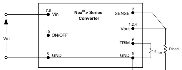
Fig. E: Configuration for programming output voltage.
