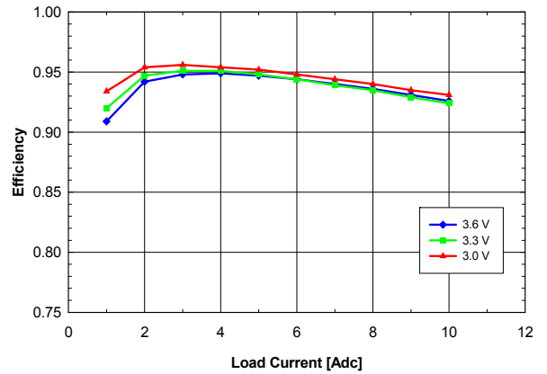
Fig. 2.0V.4: Efficiency vs. load current and input voltage for V_{out} = 2.0V converter mounted vertically with air flowing from pin 10 to pin 1 at a rate of 200 LFM (1m/s) and T_a = 25^{\circ}C .
