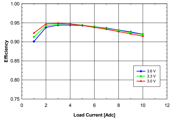
Fig. 1.8V.4: Efficiency vs. load current and input voltage for V_{out} = 1.8V converter mounted vertically with air flowing from pin 10 to pin 1 at a rate of 200 LFM (1m/s) and T_a = 25^{\circ}C .
