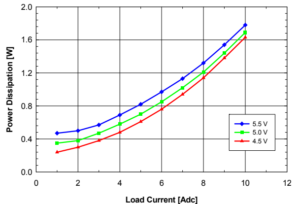
Fig. 3.3V.4: Power loss vs. load current and input voltage for V_{out} = 3.3V converter mounted vertically with air flowing from pin 10 to pin 1 at a rate of 200 LFM (1m/s) and T_a = 25^{\circ}C .
