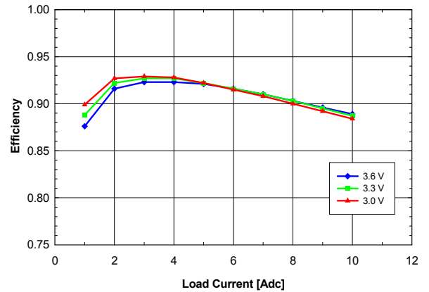
Fig. 1.2V.4: Efficiency vs. load current and input voltage for Vout = 1.2V converter mounted vertically with air flowing from pin 10 to pin 1 at a rate of 200 LFM (1m/s) and Ta = 25°C.
