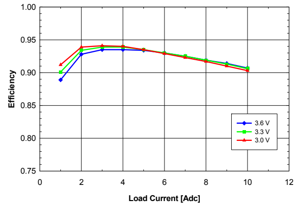
Fig. 1.5V.4: Efficiency vs. load current and input voltage for V out = 1.5V converter mounted vertically with air flowing from pin 10 to pin 1 at a rate of 200 LFM (1m/s) and T a = 25°C.
