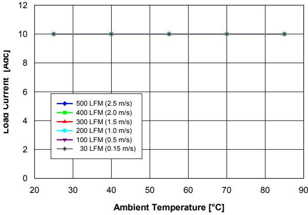
Fig. 1.2V.1: Available load current vs. ambient temperature and airflow rates for Vout = 1.2V converter mounted vertically with air flowing from pin 10 to pin 1, and maximum MOSFET temperature ≤ 120°C.
