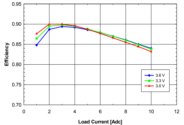
Fig. 0.7525V.4: Efficiency vs. load current and input voltage for V_{out} = 0.7525V converter mounted vertically with air flowing from pin 10 to pin 1 at a rate of 200 LFM (1m/s) and T_a = 25^{\circ}C .
