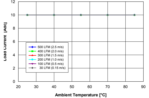
Fig. 1.5V.2: Available load current vs. ambient temperature and airflow rates for V out = 1.5V converter mounted horizontally with air flowing from pin 10 to pin 1, and maximum MOSFET temperature ≤ 120°C.
