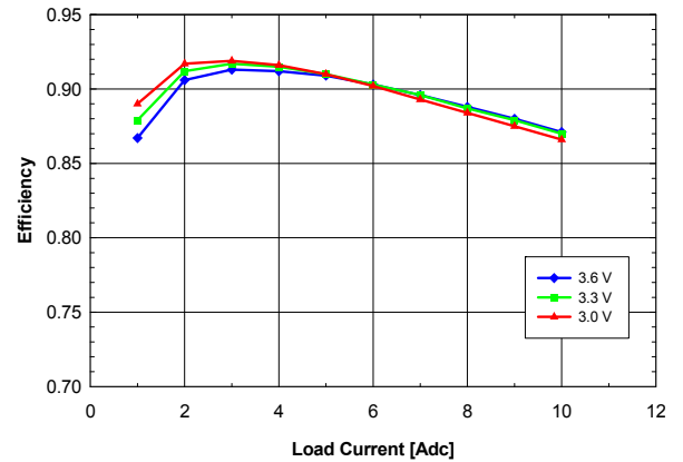
Fig. 1.0V.4: Efficiency vs. load current and input voltage for V out = 1.0V converter mounted vertically with air flowing from pin 10 to pin 1 at a rate of 200 LFM (1m/s) and T a = 25°C.
