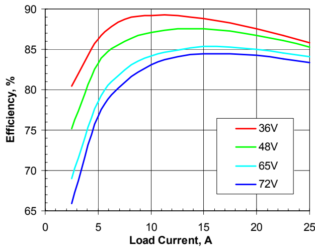
Figure 2. Efficiency vs. load current and input voltage for SSQE48T25018 converter mounted vertically with air flowing from pin 1 to pin 3 at a rate of 300 LFM (1.5 m/s) and Ta=25°C.
