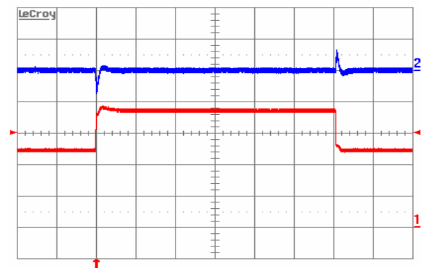
Figure 9. Output voltage response to load current step-change (12.5A-18.75A-12.5A) at V_{in}=48\text{V} . Top trace: output voltage (200 mV/div.). Bottom trace: load current (5A/div.). Current slew rate: 5A/ \mu\text{s} . C_o=470\mu\text{F POS}+1\mu\text{F cer} . Time scale: 0.2ms/div.
