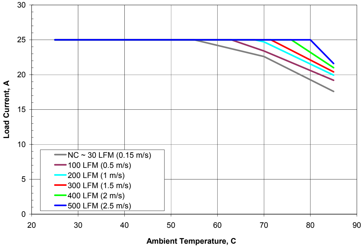
Figure 1. Available load current vs. ambient air temperature and airflow rates for SSQE48T25018 converter mounted vertically with air flowing from pin 1 to pin 3, Vin = 48 V. Note: NC – Natural convection
