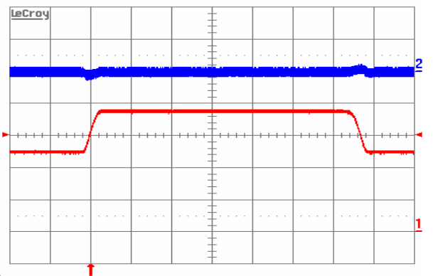
Figure 8. Output voltage response to load current step-change (12.5A-18.75A-12.5A) at V_{in}=48\text{V} . Top trace: output voltage (200mV/div.). Bottom trace: load current (5A/div.). Current slew rate: 0.1A/ \mu\text{s} . C_o=1\mu\text{F cer}+10\mu\text{F tant} . Time scale: 0.2ms/div.
