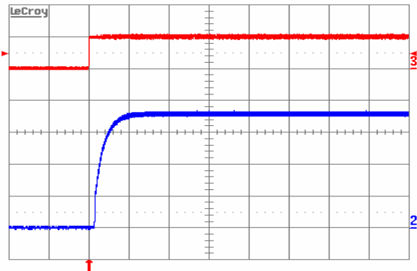
Figure 6. Turn-on transient at full rated load current (resistive) with C_o=1\mu\text{F cer}+10\mu\text{F tant} at V_{in}=48\text{V} , triggered via ON/OFF pin. Top trace: ON/OFF signal (5 V/div.). Bottom trace: Output voltage (0.5 V/div.). Time scale: 5 ms/div.
