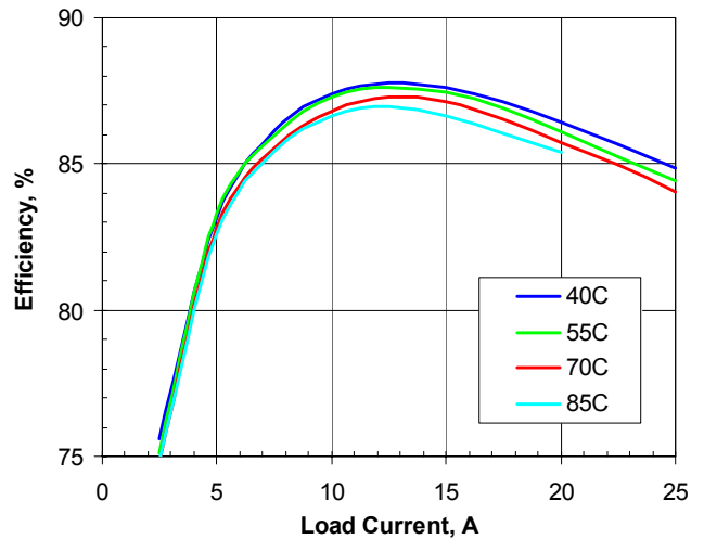
Figure 3. Efficiency vs. load current and ambient temperature for SSQE48T25018 converter mounted vertically with Vin=48V and air flowing from pin 1 to pin 3 at a rate of 200 LFM (1.0 m/s).
