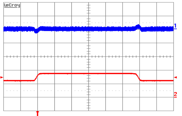
Figure 8. Output voltage response to load current step-change (12.5A-18.75A-12.5A) at V_{in}=48\text{V} . Top trace: output voltage (100mV/div.). Bottom trace: load current (10A/div.). Current slew rate: 0.1A/ \mu\text{s} . C_o=1\mu\text{F cer}+10\mu\text{F tant} . Time scale: 0.2ms/div.
