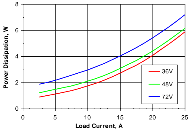
Figure 4. Power dissipation vs. load current and input voltage for SSQE48T25012 converter mounted vertically with air flowing from pin 1 to pin 3at a rate of 300 LFM (1.5 m/s) and T_a = 25\text{ }^\circ\text{C} .
