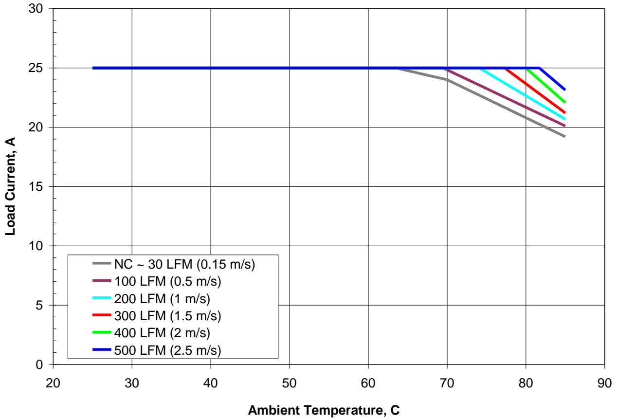
Figure 1. Available load current vs. ambient air temperature and airflow rates for SSQE48T25012 converter mounted vertically with air flowing from pin 1 to pin 3, V_{in} = 48\text{ V} . Note: NC – Natural convection
