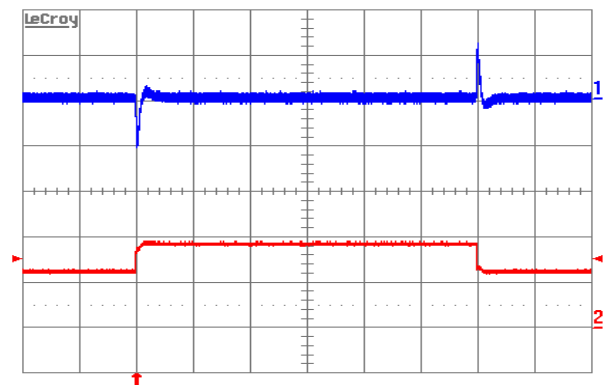
Figure 9. Output voltage response to load current step-change (12.5A-18.75A-12.5A) at V_{in}=48\text{V} . Top trace: output voltage (100 mV/div.). Bottom trace: load current (10A/div.). Current slew rate: 5A/ \mu\text{s} . C_o=470\mu\text{F POS}+1\mu\text{F cer} . Time scale: 0.2ms/div.
