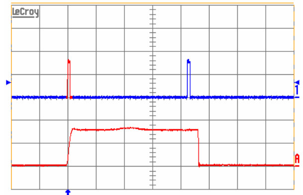
Figure 15. Load current (top trace, 10 A/div., 50 ms/div.) into a 10 \text{ m}\Omega short circuit during restart, at V_{in} = 48 \text{ V} . Bottom trace (10 A/div., 1.0 ms/div.) is an expansion of the on-time portion of the top trace
