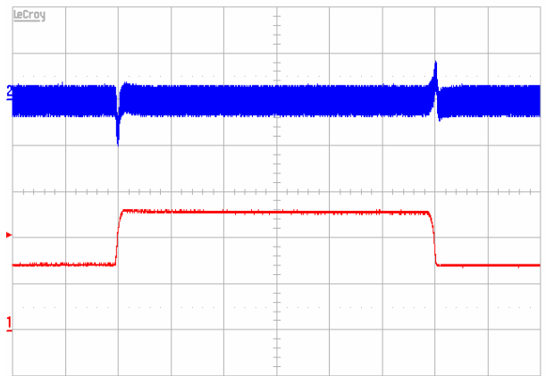
Figure 8. Output voltage response to load current step-change (3.5A–5.25A–3.5A) at V_{in}=48\text{V} . Top trace: Vout (100 mV/div.). Bottom trace: Iout (2 A/div.), Time: (0.2 ms/div.) Current slew rate: 0.1 A/ \mu\text{s} . C_o=1\mu\text{F} ceramic + 10 \mu\text{F} tantalum.
