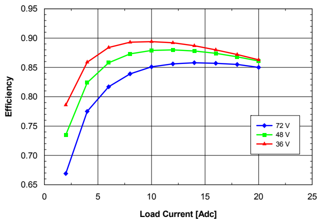
Fig. 1.8V.2: Efficiency vs. load current and input voltage for SQM48T/S20018 converter mounted vertically with air flowing from pin 3 to pin 1 at a rate of 300 LFM (1.5 m/s) and T_a = 25\text{ }^\circ\text{C} .
