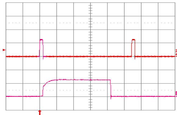
Fig. 1.5V.12: Load current (top trace, 20 A/div., 20 ms/div.) into a 10 mΩ short circuit during restart, at V in = 48 V. Bottom trace (20 A/div., 1 ms/div.) is an expansion of the on-time portion of the top trace.
