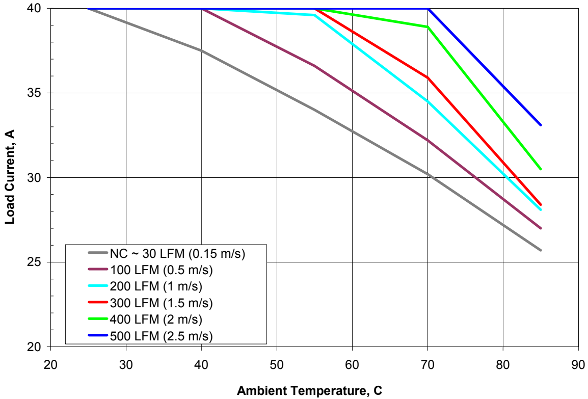
Figure 1. Available load current vs. ambient air temperature and airflow rates for SQE48T40018 converter mounted vertically with air flowing from pin 3 to pin 1, MOSFET temperature \leq 120^\circ\text{C} , V_{in} = 48\text{ V} . Note: NC – Natural convection
