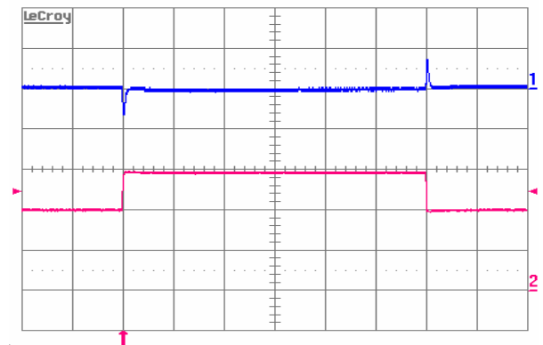
Figure 9. Output voltage response to load current step-change (20A – 30A – 20A) at V_{in} = 48\text{ V} . Top trace: output voltage (200 mV/div.). Bottom trace: load current (10 A/div.). Current slew rate: 2.5A/ \mu\text{s} . C_o = 470\ \mu\text{F} POS + 1 \mu\text{F} ceramic. Time scale: 0.2 ms/div.
