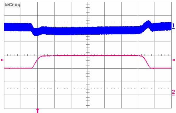
Figure 8. Output voltage response to load current step-change (20 A – 30 A – 20 A) at V_{in} = 48\text{ V} . Top trace: output voltage (50 mV/div.). Bottom trace: load current (10 A/div.). Current slew rate: 0.1 A/ \mu\text{s} . C_o = 1\ \mu\text{F} ceramic. Time scale: 0.2ms/div.
