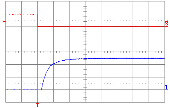
Fig. 2.5V.8: Turn-on transient at full rated load current (resistive) plus 10,000 µF at V_{in} = 48\text{ V} , triggered via ON/OFF pin. Top trace: ON/OFF signal (5 V/div.). Bottom trace: Output voltage (1 V/div.). Time scale: 2 ms/div.
