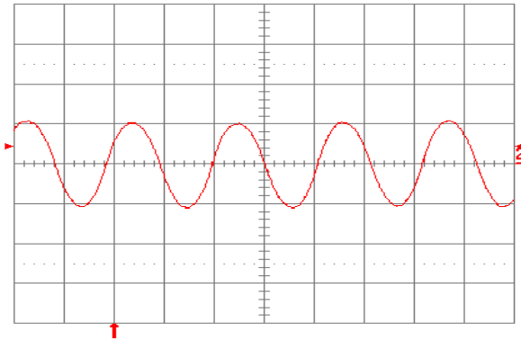
Fig. 2.5V.13: Input reflected-ripple current, i_c (100 mA/div.), measured at input terminals at full rated load current and V_{in} = 48 V. Refer to Fig. 2.5V.12 for test setup. Time scale: 1 \mu s/div.
