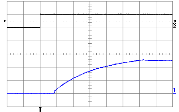
Fig. 5.0V.10: Turn-on transient at full rated load current (resistive) plus 10,000 µF at V_{in} = 48\text{V} , triggered via ON/OFF pin. Top trace: ON/OFF signal (5 V/div.). Bottom trace: output voltage (2 V/div.). Time scale: 2ms/div.
