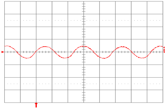
Fig. 2.5V.15: Input reflected ripple current, i_c (100 mA/div.), measured at input terminals at full rated load current and V_{in} = 48 V. Refer to Fig. 2.5V.14 for test setup. Time scale: 1 \mu s/div.
