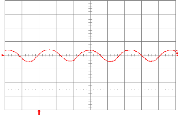
Fig. 2.0V.15: Input reflected ripple current, i_c (100 mA/div.), measured at input terminals at full rated load current and V_{in} = 48 V. Refer to Fig. 2.0V.14 for test setup. Time scale: 1 \mu s/div.
