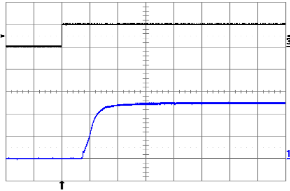
Fig. 5.0V.9: Turn-on transient at full rated load current (resistive) with no output capacitor at V_{in} = 48\text{V} , triggered via ON/OFF pin. Top trace: ON/OFF signal (5 V/div.). Bottom trace: output voltage (2 V/div.). Time scale: 2ms/div.
