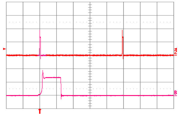
Fig. 5.0V.18: Load current (top trace, 10A/div., 20 ms/div.) into a 10 m\Omega short circuit during restart, at V_{in} = 48V . Bottom trace (10A/div., 1ms/div.) is an expansion of the on-time portion of the top trace.
