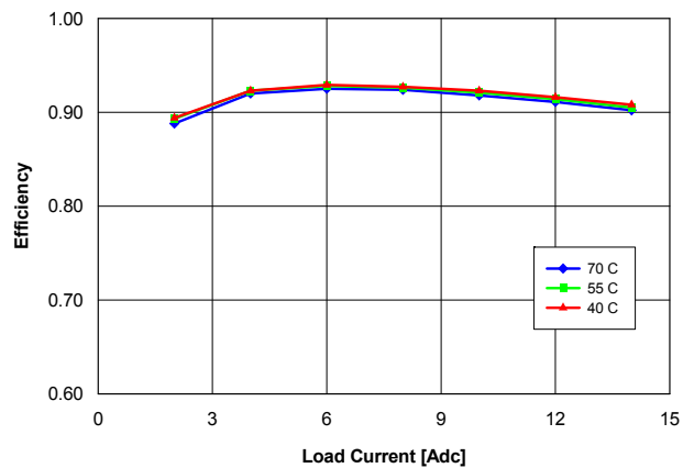
Fig. 4: Efficiency vs. load current and ambient temperature for converter mounted horizontally with V_{in} = 48\text{ V} and air flowing from pin 3 to pin 1 at a rate of 200 LFM (1.0 m/s).
