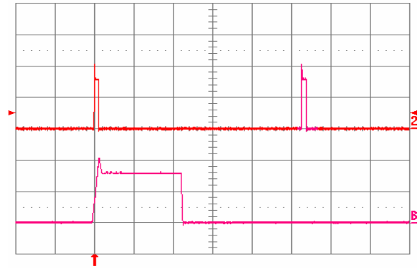
Fig. 22: Load current (top trace, 10 A/div., 20 ms/div.) into a 10 mΩ short circuit during restart, at Vin = 48 V. Bottom trace (10 A/div., 1 ms/div.) is an expansion of the on-time portion of the top trace.
