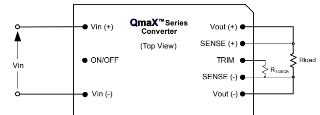
Fig. D: Configuration for decreasing output voltage.
