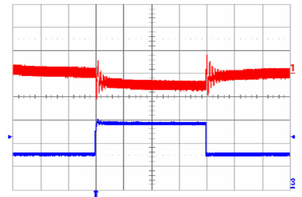
Fig. 12: Step Load response to 50% – 100% – 50% with 20 \mu F external ceramic capacitor and di/dt = 10 A/ \mu s. Top trace: output voltage (500 mV/div.). Bottom trace: load current (5 A/div.). Time scale: 0.2 ms/div.
