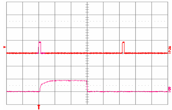
Fig. 14: Load current (top trace, 20 A/div., 20 ms/div.) into a 10 mΩ short circuit during restart, at V_{in} = 48 V. Bottom trace (10 A/div., 1 ms/div.) is an expansion of the on-time portion of the top trace.
