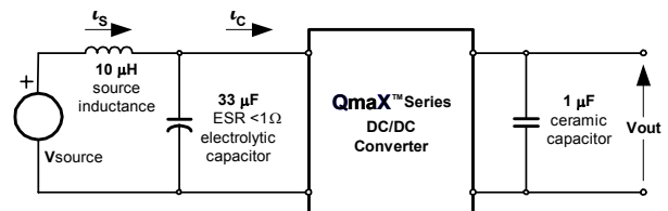
Fig. I: Test Setup for measuring input reflected-ripple currents, i_c and i_s .
