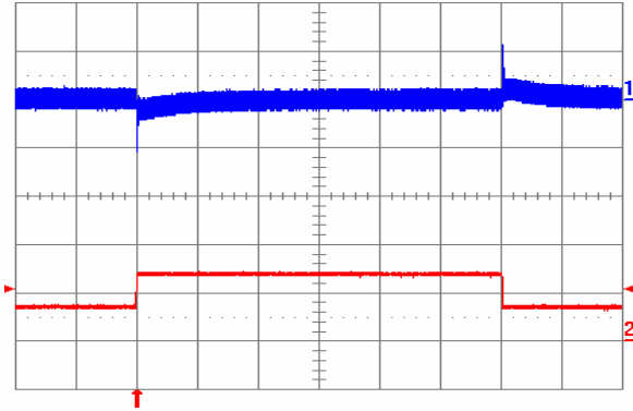
Fig. 9: Output voltage response to load current step-change (3.5 A – 7 A – 3.5 A) at V_{in} = 48 V. Top trace: output voltage (200 mV/div.). Bottom trace: load current (2 A/div.). Bottom trace: load current (5 A/div.). Current slew rate: 5 A/ \mu s. C_o = 1 \mu F ceramic. Time scale: 0.2 ms/div.
