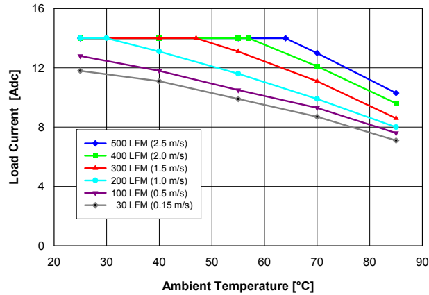
Fig. 1: Available load current vs. ambient air temperature and airflow rates for converter with B height pins mounted vertically with air flowing from pin 3 to pin 1, MOSFET temperature \leq 120^\circ\text{C} , V_{in} = 48\text{ V} .
