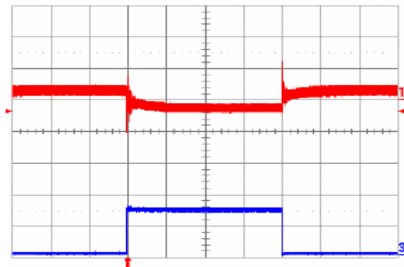
Fig. 11: Step Load response to 0% – 50% – 0% with 20 \mu F external ceramic capacitor and di/dt = 10 A/ \mu s. Top trace: output voltage (500 mV/div.). Bottom trace: load current (5 A/div.). Time scale: 0.5 ms/div.
