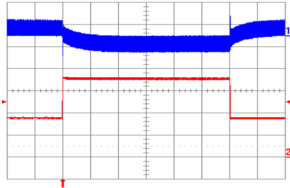
Fig. 9: Output voltage response to load current step-change (3.5 A – 7 A – 3.5 A) at V_{in} = 56 V. Top trace: output voltage (200 mV/div.). Bottom trace: load current (2 A/div.). Bottom trace: load current (5 A/div.). Current slew rate: 5 A/ \mu s. C_o = 1 \mu F ceramic. Time scale: 0.5 ms/div.
