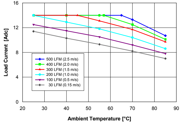
Fig. 2: Available load current vs. ambient air temperature and airflow rates for converter with B height pins mounted horizontally with air flowing from pin 3 to pin 1, MOSFET temperature \leq 120^\circ\text{C} , V_{in} = 48\text{ V} .
