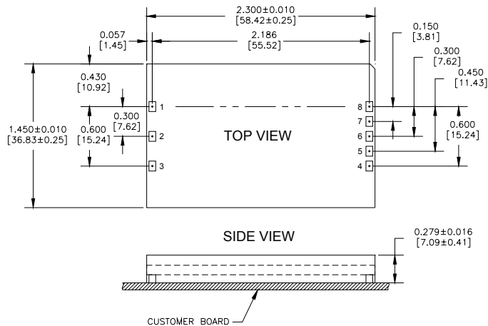
QM48S (Surface-mount)
