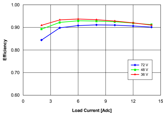
Fig. 3: Efficiency vs. load current and input voltage for converter mounted horizontally with air flowing from pin 3 to pin 1 at a rate of 300 LFM (1.5 m/s) and T_a = 25\text{ }^{\circ}\text{C} .
