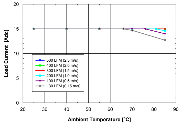
Fig. 10: Available load current vs. ambient air temperature and airflow rates for ASQ48T15018 converter with D height pins mounted horizontally with V_{in} = 48 V, air flowing from pin 3 to pin 1 and maximum FET temperature \leq 120^{\circ}\text{C} .
