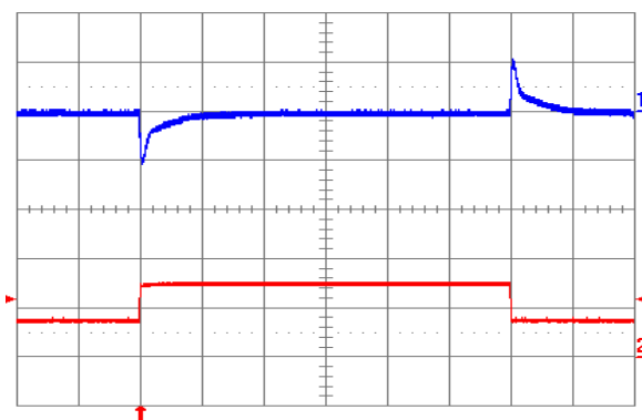
Fig. 20: Output voltage response to load current step-change (3.75 A – 7.5 A – 3.75 A) at V_{in} = 48 V. Top trace: output voltage (100 mV/div.). Bottom trace: load current (5 A/div.). Current slew rate: 5 A/ \mu s. C_o = 450 \mu F tantalum + 1 \mu F ceramic. Time scale: 0.2 ms/div.
