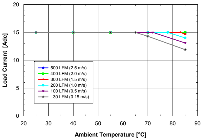
Fig. 1: Available load current vs. ambient air temperature and air-flow rates for ASQ48T15018 converter with D height pins mounted vertically with air flowing from pin 3 to pin 1, MOSFET temperature \leq 120^{\circ}\text{C} , V_{in} = 48\text{ V} .
