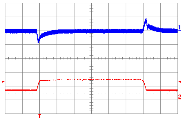
Fig. 19: Output voltage response to load current step-change (3.75 A – 7.5 A – 3.75 A) at V_{in} = 48 V. Top trace: output voltage (100 mV/div.). Bottom trace: load current (5 A/div.). Current slew rate: 0.1 A/ \mu s. C_o = 1 \mu F ceramic. Time scale: 0.2 ms/div.
