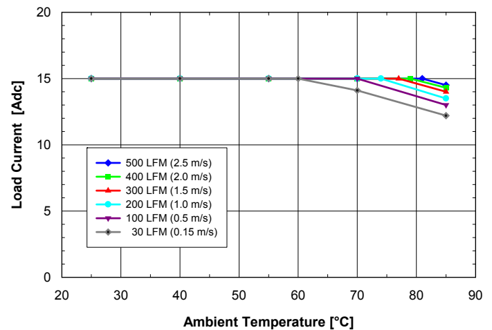
Fig. 12: Available load current vs. ambient temperature and airflow rates for ASQ48S15018 converter mounted horizontally with V_{in} = 48 V, air flowing from pin 3 to pin 1 and maximum FET temperature \leq 120^{\circ}\text{C} .
