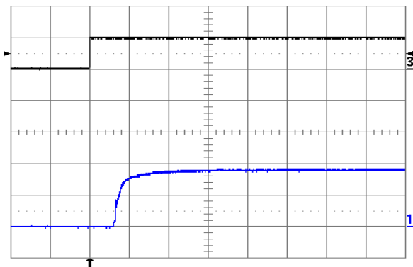
Fig. 17: Turn-on transient at full rated load current (resistive) with no output capacitor at V_{in} = 48 V, triggered via ON/OFF pin. Top trace: ON/OFF signal (5 V/div.). Bottom trace: output voltage (1 V/div.) Time scale: 2 ms/div.
