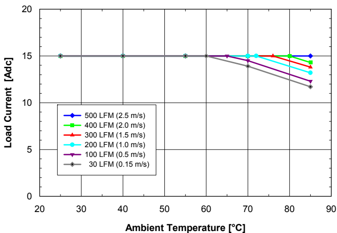
Fig. 11: Available load current vs. ambient temperature and airflow rates for ASQ48S15018 converter mounted vertically with V_{in} = 48 V, air flowing from pin 3 to pin 1 and maximum FET temperature \leq 120^{\circ}\text{C} .
