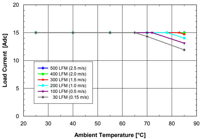
Fig. 9: Available load current vs. ambient air temperature and airflow rates for ASQ48T15018 converter with D height pins mounted vertically with V_{in} = 48 V, air flowing from pin 3 to pin 1 and maximum FET temperature \leq 120^{\circ}\text{C} .
