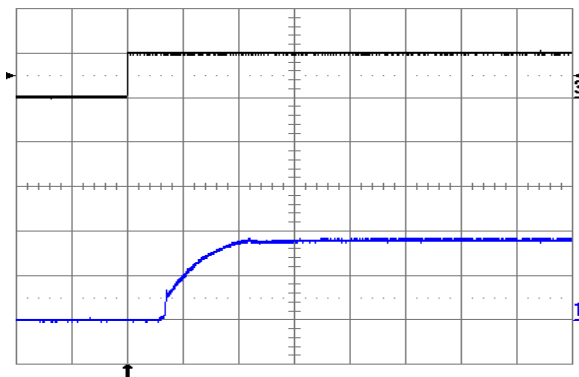
Fig. 18: Turn-on transient at full rated load current (resistive) plus 10,000 \mu F at V_{in} = 48 V, triggered via ON/OFF pin. Top trace: ON/OFF signal (5 V/div.). Bottom trace: output voltage (1 V/div.). Time scale: 2 ms/div.
