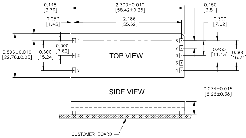
ASQ28S Pinout (Surface Mount)
