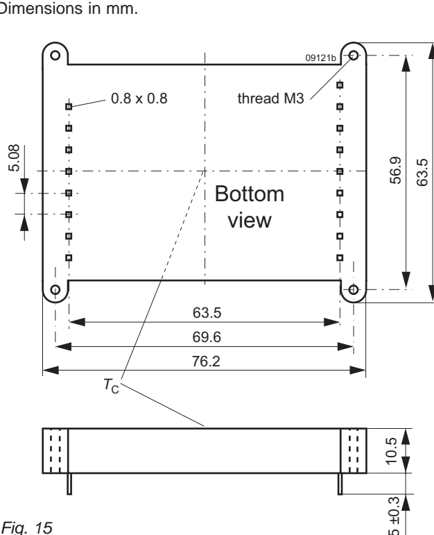
Fig. 15 Case IMX35 (Standard) Weight: approx. 67 g
