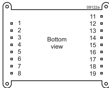
Fig. 17 Footprint. The holes in the PCB should have a diameter of 1.5 mm.
