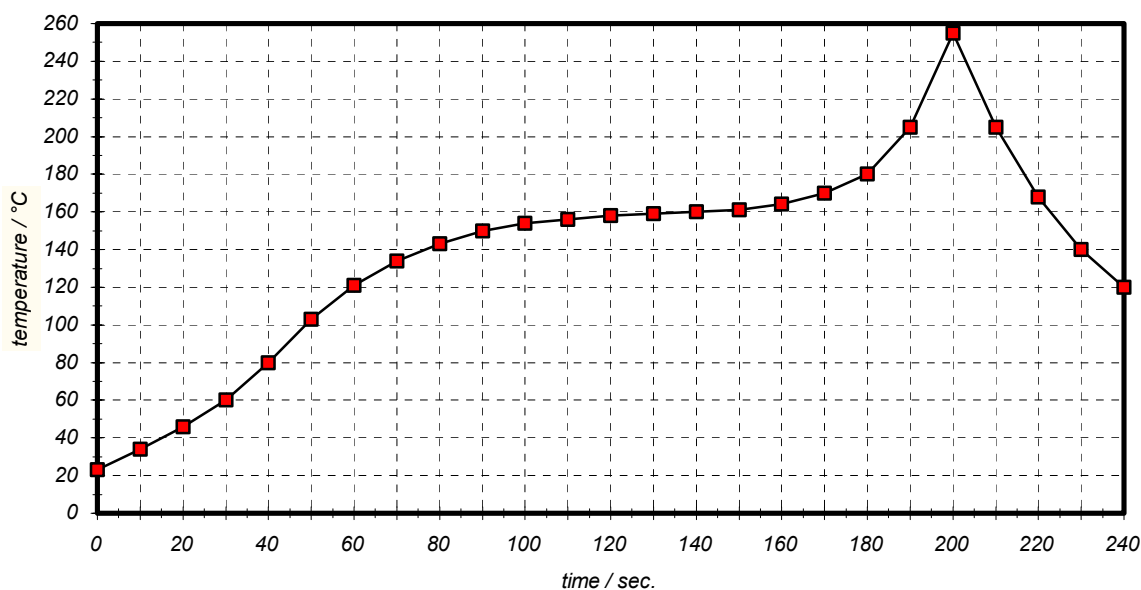
Chip-mount air reflow profile
