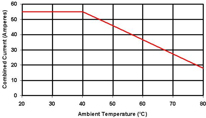
HS103DR w/50A 3-Phase SSR
