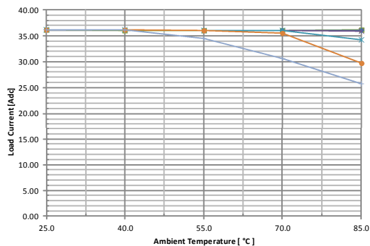
Fig. 5: Available load current vs. ambient air temperature and airflow rates for UIE48T36033 converter with baseplate equipped with .45" finned heatsink mounted vertically with air flowing from pin 3 to pin 1, MOSFET temperature \leq 125^{\circ}\text{C} , V_{in}=48\text{V}
