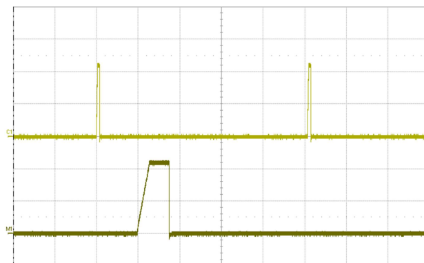
Fig. 17: Load current (top trace, 20\ \text{A}/\text{div} , 100\ \text{ms}/\text{div} .) into a 10\ \text{m}\Omega short circuit during restart, at V_{in} = 48\ \text{V} . Bottom trace ( 20\ \text{A}/\text{div} , 10\ \text{ms}/\text{div} .) is an expansion of the on-time portion of the top trace
