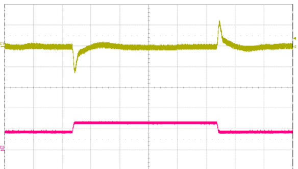
Fig. 12: Output voltage response to load current step change (18A – 27A – 18A) at V_{in} = 48 \text{ V} . Top trace: output voltage (200 mV/div.). Bottom trace: load current (20 A/div.). Current slew rate: 1 \text{ A}/\mu\text{s} . C_o = 1 \mu\text{F} ceramic + 10,000 \mu\text{F} + 10 \mu\text{F} tantalum. Time scale: 200 \mu\text{s}/\text{div} .
