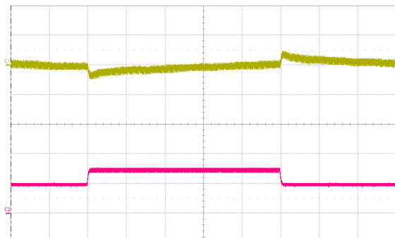
Fig. 12: Output voltage response to load current step-change (5 A – 7.5A – 5 A) at V_{in} = 48\text{ V} . Top trace: output voltage (500 mV/div.). Bottom trace: load current (5 A/div.). Current slew rate: 1 A/ \mu\text{s} . C_o = 1\ \mu\text{F} ceramic + 4,700 \mu\text{F} + 10 \mu\text{F} tantalum. Time scale: 200 \mu\text{s} /div.
