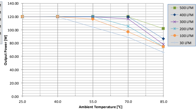
Fig. 2: Power derating vs. ambient air temperature and airflow rates for UIE48T10120 converter w/o baseplate mounted vertically with air flowing from pin 3 to pin 1, MOSFET temperature \leq 125^{\circ}\text{C} , V_{in}=48\text{V} .
