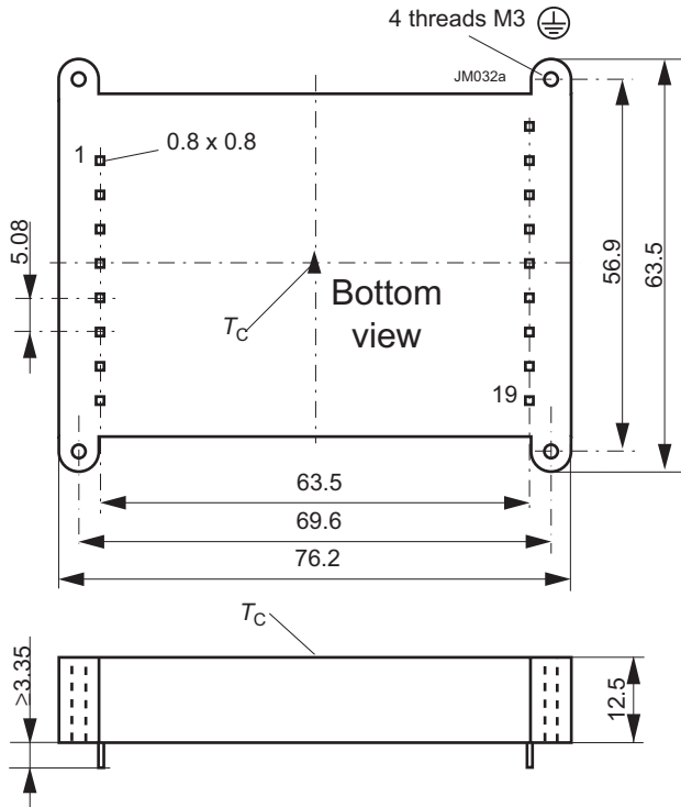
Fig. 13 Case IMX70/IMY70 (Standard) Weight: approx. 130 g
