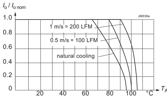
Fig. 6b Maximum allowed output power versus ambient temperature for 24IMX70-24-24 with option Z in vertical position.
