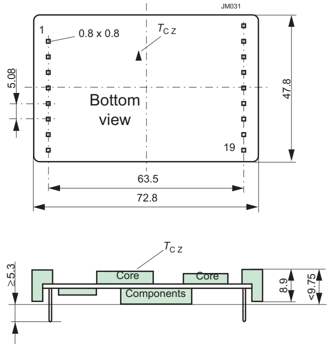
Fig. 14 IMX70/IMY70 open frame (option Z) Weight: approx. 60 g
