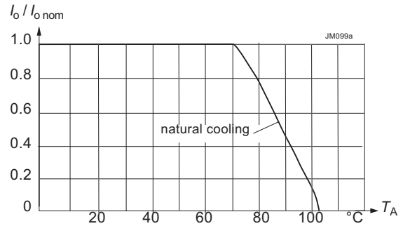
Fig. 6c Maximum allowed output power versus ambient temperature for converters 110IMY70-12 with option Z in vertical position.
