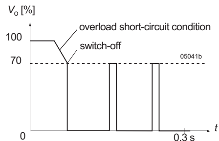
Fig. 8 Current limitation of single-output models or double-output models with both outputs connected in parallel
