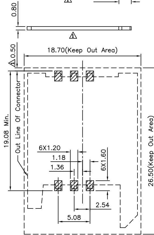
Recommended P.C.B. Layout General Tolerance:±0.05
