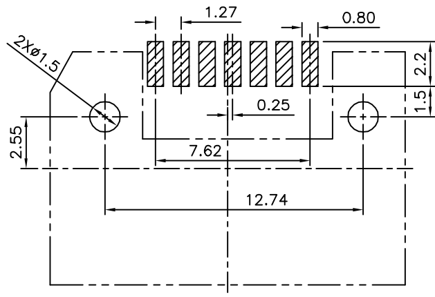
△ Recommended P.C.B. Layout(Top Side) (PCB Thickness:1.60mm)
