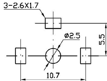
Dimensions of PC board holes (Commend)
