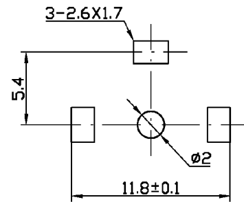
Dimensions of PC board holes (Commend)
