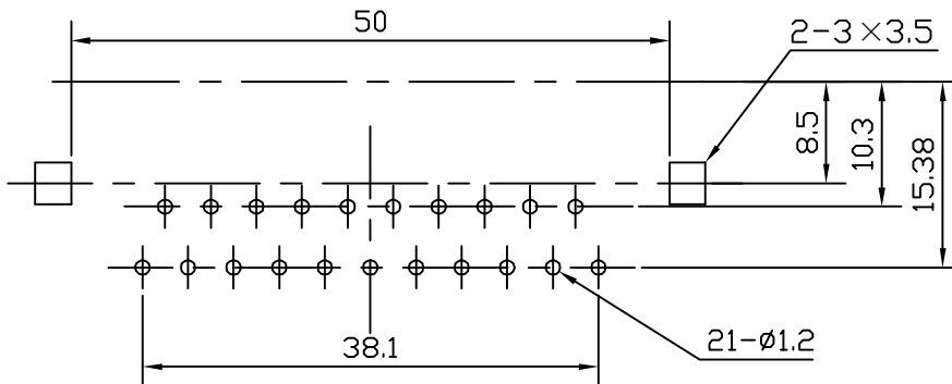
Dimensions of PC board holes
