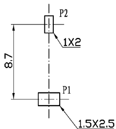
Dimensions of PC board holes (Commend)
