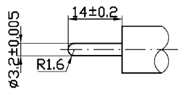
Gauge Plug
